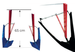
ADJUSTABLE BLADE TO WEED BETWEEN RIDGES
