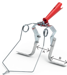
SPACING BETWEEN THE BLADES (A): 90mm/120mm
